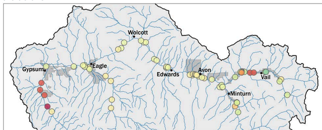
Percent Change in Annual 7-Day Min Streamflow -100 to -50 -50 to -20 -20 to -10 -10 to -5 -5 to 0 0 to 5 5 to 10 10 to 20 20 to 50
