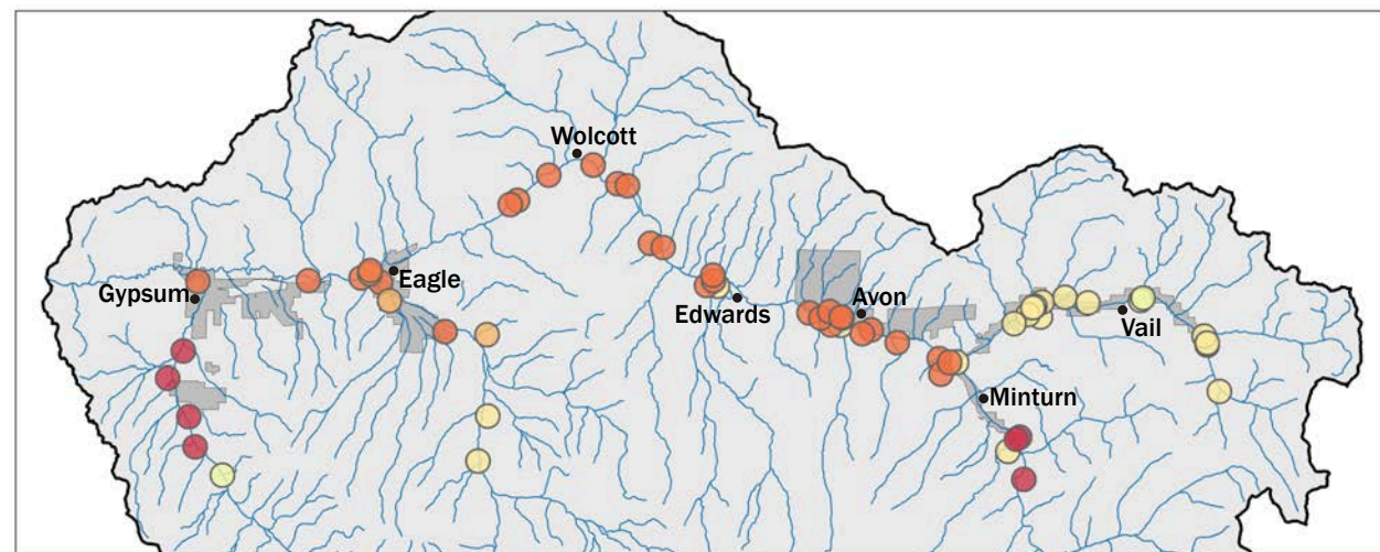
Percent Change in Annual 3-Day Max Streamflow -50 to -20 -20 to -10 -10 to -5 -5 to 0 0 to 5 5 to 10 10 to 20
